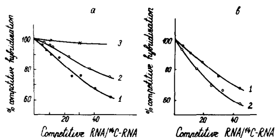
Fig.2. Competitive hybridization. Comparison of normal liver RNA (1) with that from liver nuclei of rats treated with DAB for 1 day. (2) [ ^{14}\text{C} ] -Labelled RNA from normal (a) and DAB-treated liver (b), 5 \mu\text{g} , was incubated in 0.2 ml of 0.24 MPB, pH 6.8, with the fraction of unique DNA, 300 \mu\text{g} , Cot = 5000 , in the presence of increasing amounts of unlabelled competing RNA. (3) Unspecific hybridization; competitor-cytoplasmic RNA from E. coli . Abscissa: the ratio of the amount of competitive RNA to [ ^{14}\text{C} ] RNA in a hybridization sample. Ordinate: percent of competitive hybridization (hybridization in the absence of competitor is taken for 100%).
