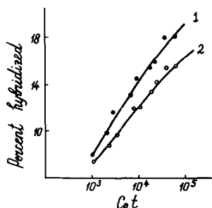
Fig.1. Hybridization capacity of nuclear [ ^{14}\text{C} ] RNA isolated from livers of control (1) and DAB-treated rats (2) with the fraction of slowly renaturing DNA. 2–3 \mu\text{g} [ ^{14}\text{C} ] RNA was incubated in 0.1–0.2 ml of 0.24 M PB, the ratio DNA/RNA = 150. Abscissa: Cot value. Ordinate: percent of hybridization.
